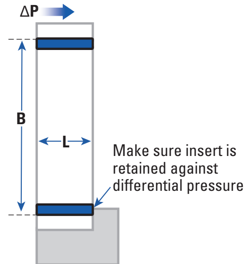
B. Inside diameter of stationary bore L. Length of bore \Delta P . Direction of differential pressure
