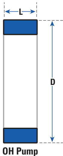
D. Diameter of existing case ring L. Overall part length
