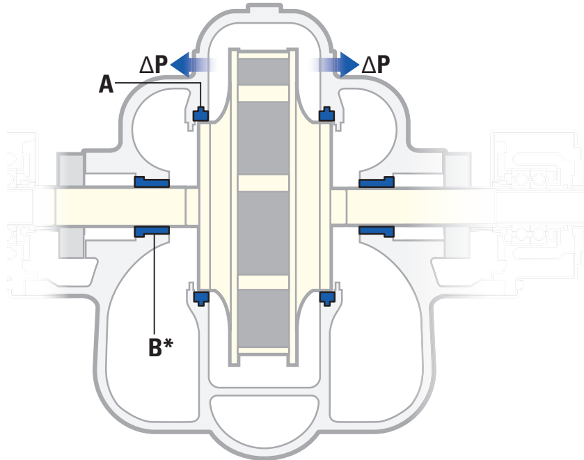
A. Case Wear Rings B. Throat Bushings \Delta P . Direction of differential pressure *Direction of differential pressure across throat bushing to be confirmed by seal OEM
