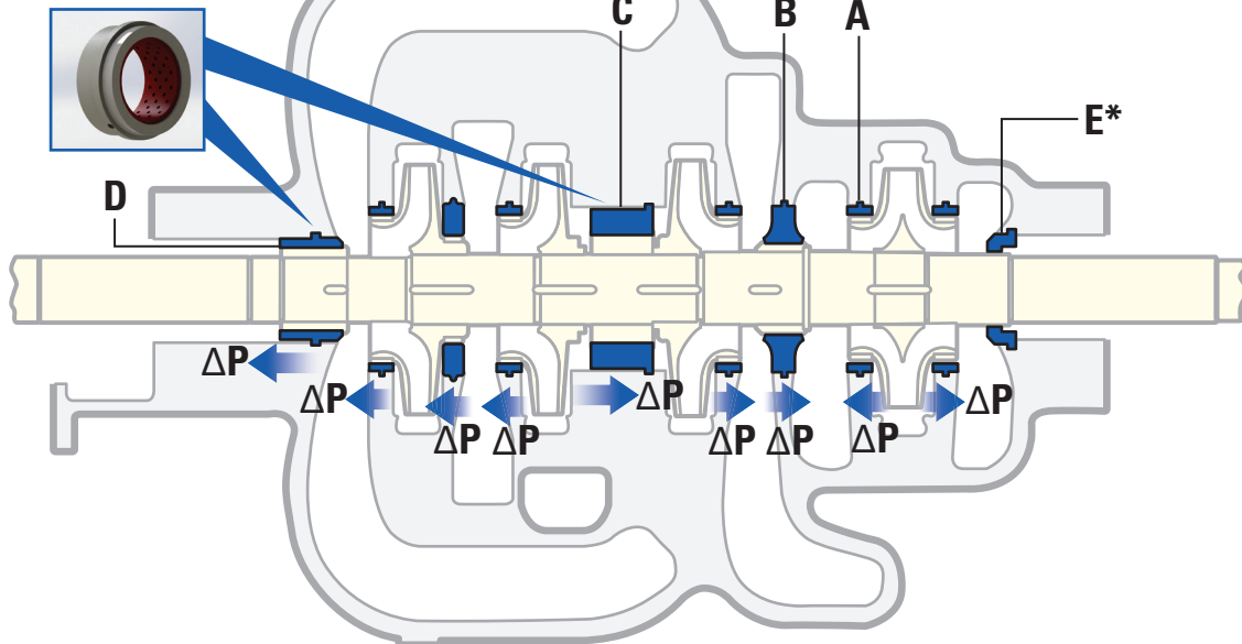
A. Case Wear Rings B. Inter-stage Rings C. Center Bushings D. Throttle Bushings E. Throat Bushings \Delta P . Direction of differential pressure *Direction of differential pressure across throat bushing to be confirmed by seal OEM
